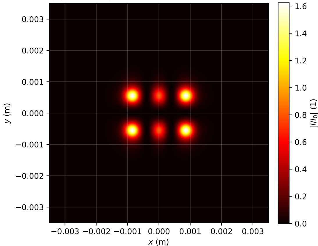
Intensity profile I(x, y, z = 0.716)/I_0 , P_{in}=3.0P_{cr} , artificial time
